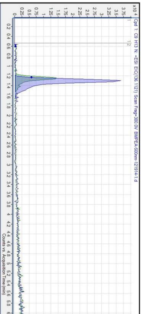
Figure 2. Extracted ion chromatograms of BMPEA (500 ng/mL, lighter) and amphetamine-d5 (100 ng/mL, darker).
